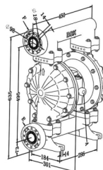
Plastic pump
