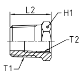
REDUCER BUSHING
